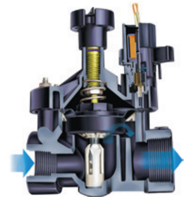
PESB Cutaway
